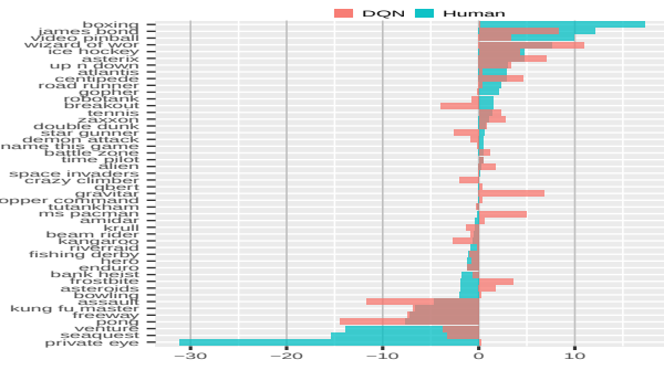
Figure 3: Comparison of RAS Rollout IW(1) with time budget of 0.5 seconds with the human player and DQN using relative scores over 48 games. Blue bars depict RAS Rollout IW(1) scores ( r ) vs. human scores ( h ), while red bars, RAS Rollout IW(1) scores vs. DQN scores ( d ). The bar has positive length (r - h)/h when r > h , and negative length (h - r)/r when r < h . Bars have zero length when r = h . Same for d in place of h .
